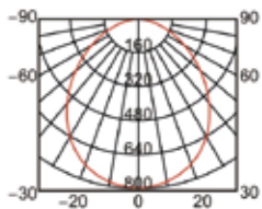
Light distribution(灯具配光曲线)
