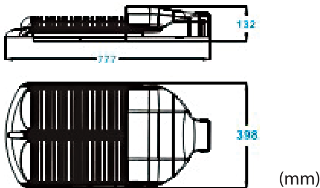
Product Dimension
